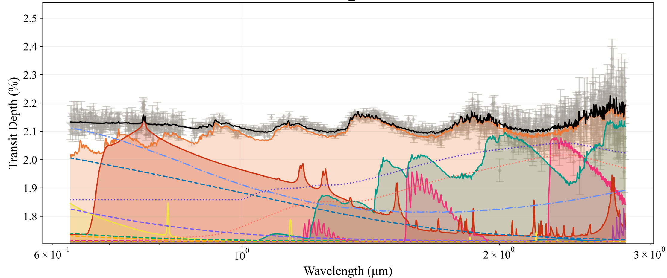
niriss_SiO
